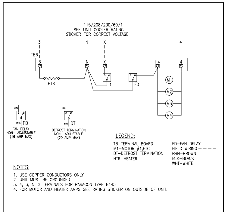
Electric Defrost Wiring
