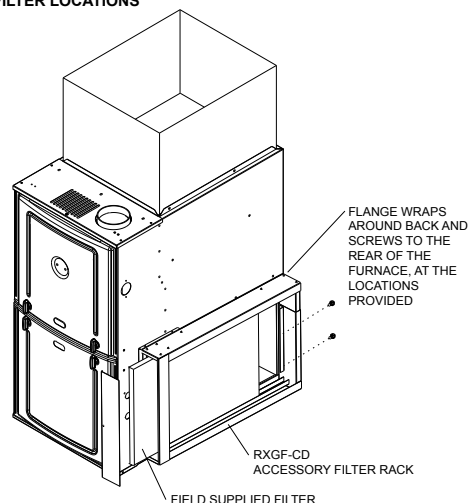
FIGURE 4 UPFLOW – RECOMMENDED
