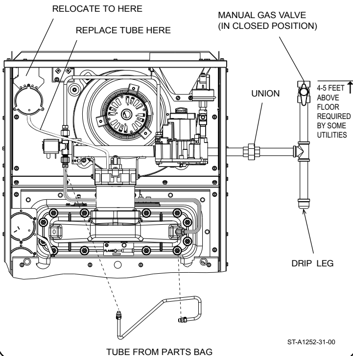
FIGURE 2B ALTERNATE GAS PIPING INSTALLATION
