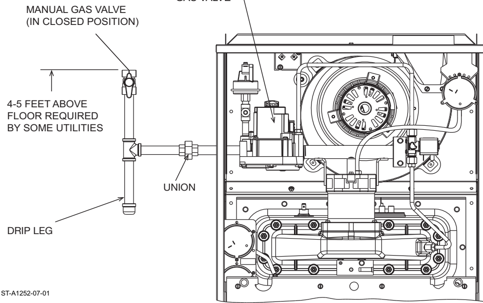
FIGURE 2 GAS PIPING INSTALLATION
