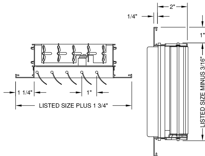
MODEL - C1SO - 1 WAY SHORT - OPPOSED BLADE DAMPER
