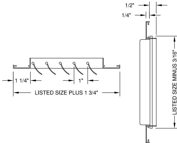
MODEL - C1S - 1 WAY SHORT - GRILLE
