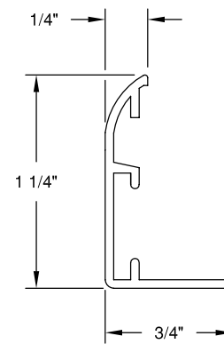
MODEL - C1SM - 1 WAY SHORT - MULTI-SHUTTER DAMPER
