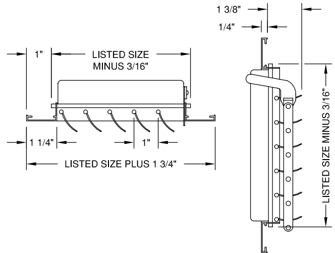
MODEL - C1SM - 1 WAY SHORT - MULTI-SHUTTER DAMPER
