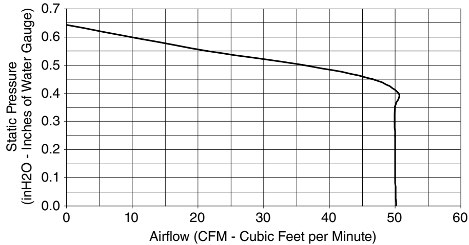
XN50 - 4" DUCT
