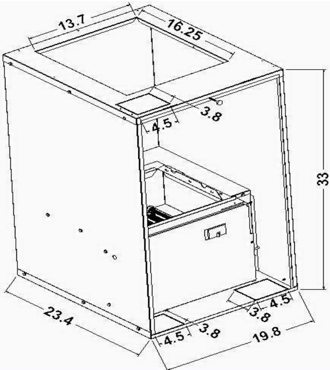
Figure 1: Furnace Dimensions
