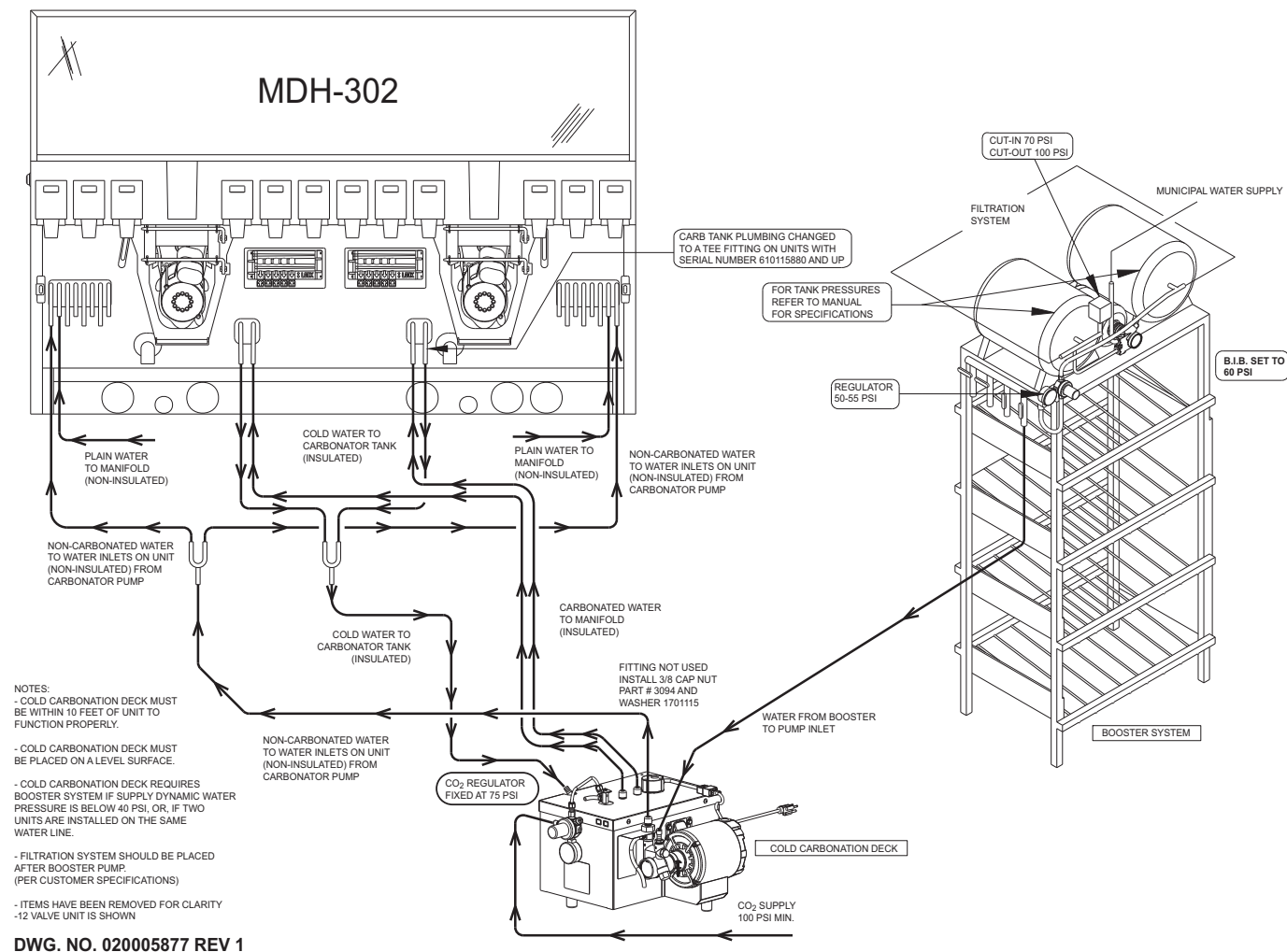
Typical MDH-302 Cold Carbonation Beverage Dispensing System
