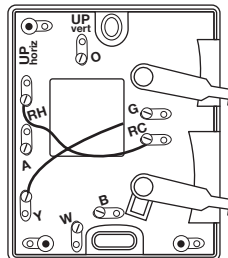
FIGURE 3 SUB-BASE
