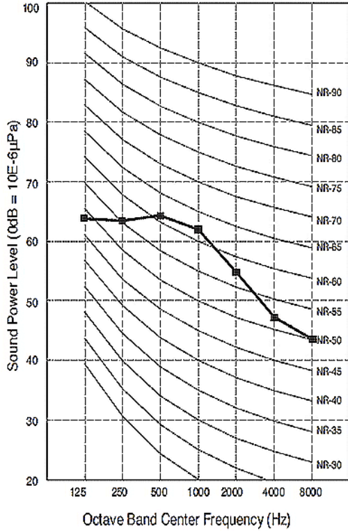
Figure 25: LUU428HV, LUU488HV Sound Power Level Diagram.
