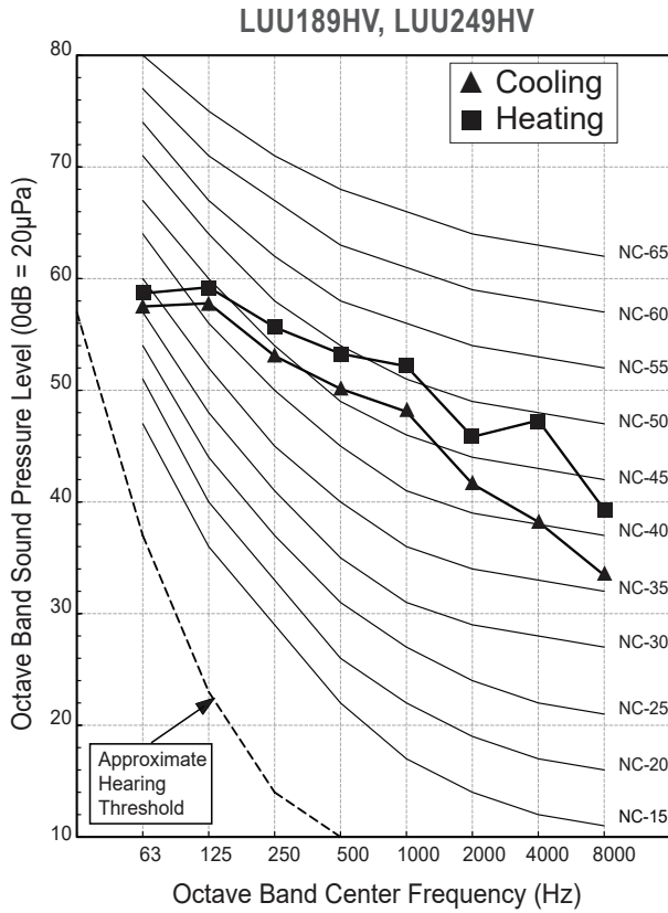
Figure 20: LUU189HV, LUU249HV Sound Pressure Level Diagram.
