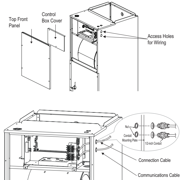
Figure 36: Connecting the Power Wiring and Communications Cable.
