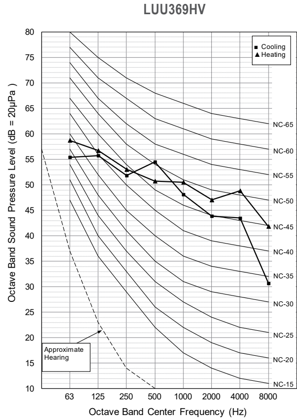
Figure 21: LUU369HV Sound Pressure Level Diagram.
