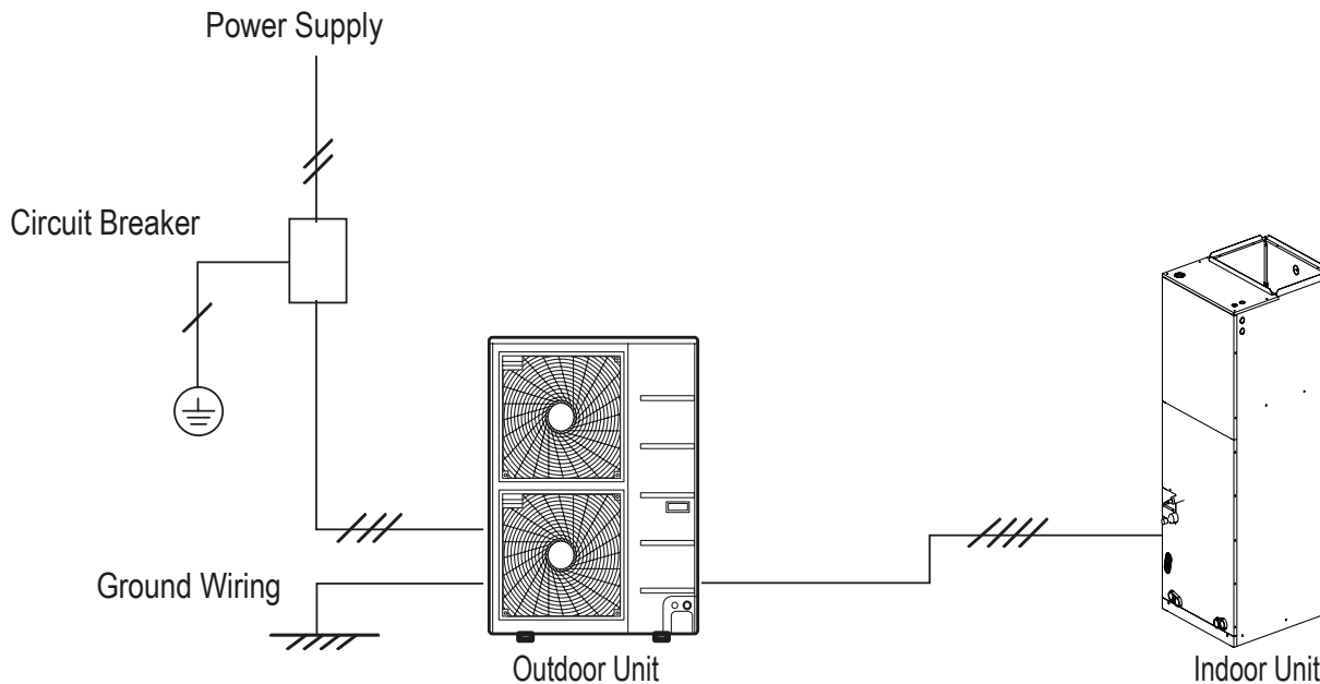
Figure 35: LV361HV4, LV480HV, and LV488HV General Power/Communications System Schematic.
