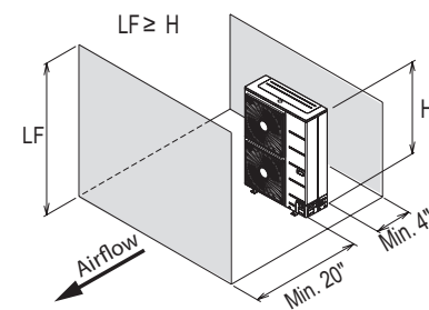
Figure 60: Proper Outdoor Unit Placement and Clearances, continued.
