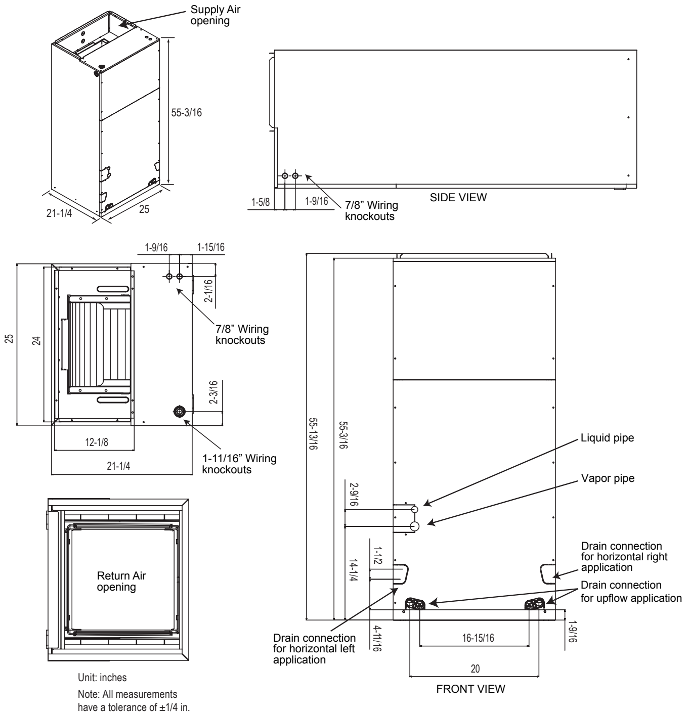
Figure 7: LVN420HV, LVN480HV Indoor Unit Dimensions.
