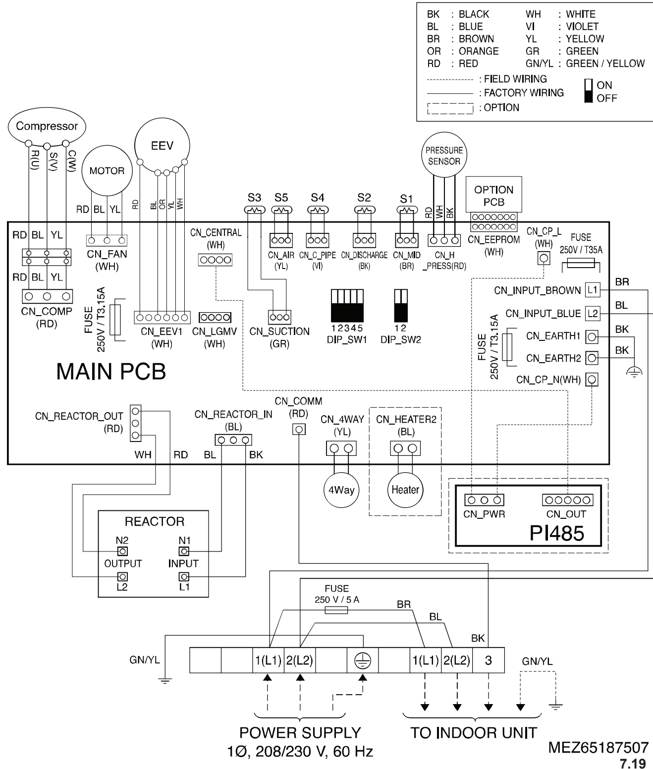
Figure 31: Outdoor Unit Wiring Diagram.
