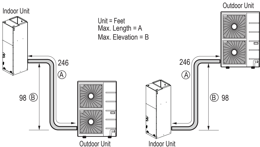
Figure 64: Typical LV361HV4, LV420HV and LV480HV System Layout.
