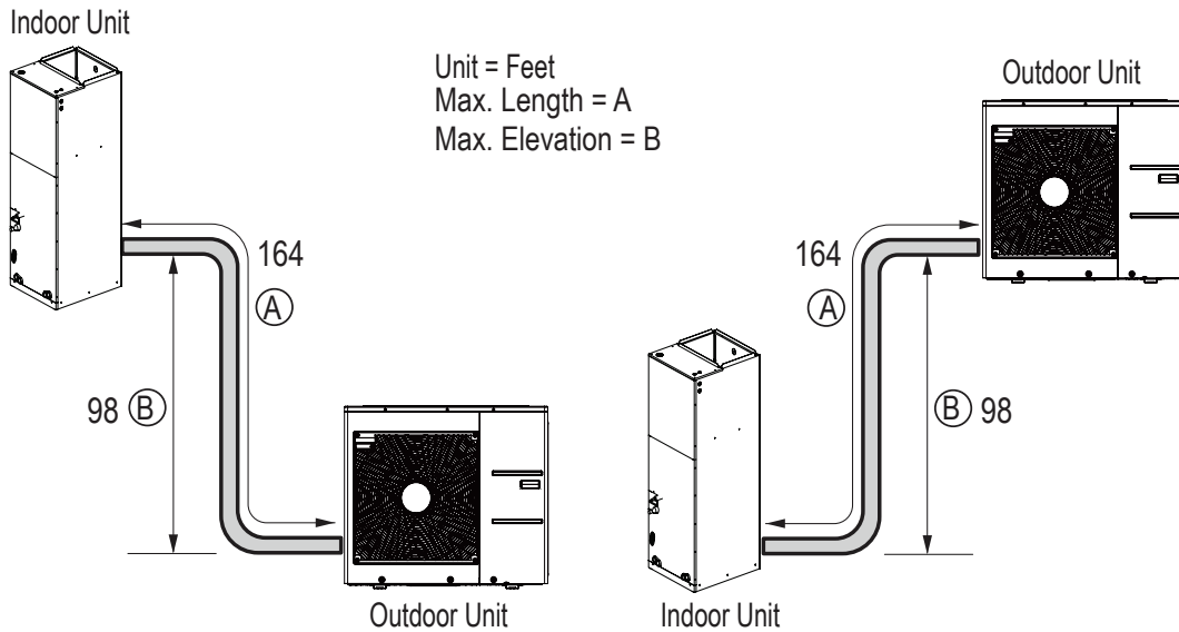
Figure 63: Typical LV181HV4 and LV241HV4 System Layout.
