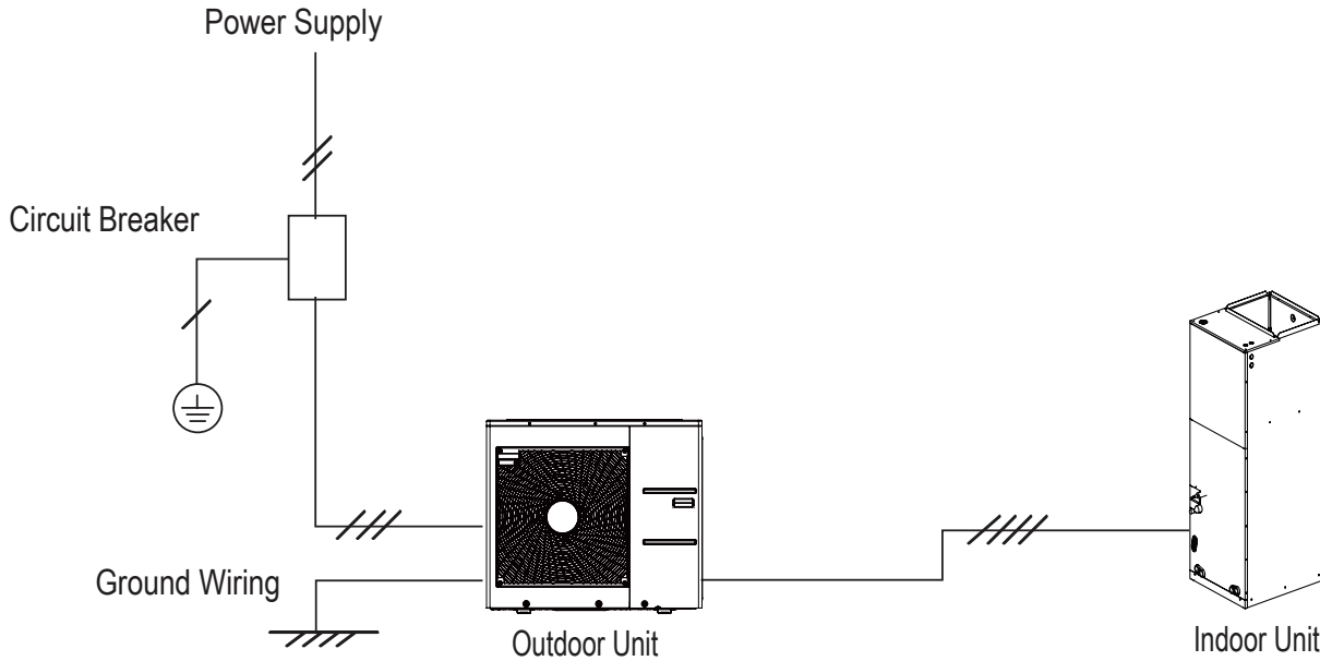
Figure 35: LV361HV4, LV480HV, and LV488HV General Power/Communications System Schematic.
