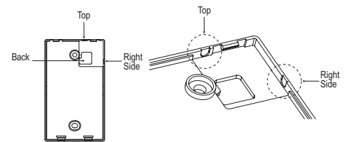
Figure 43: Installing / Removing the Controller.
