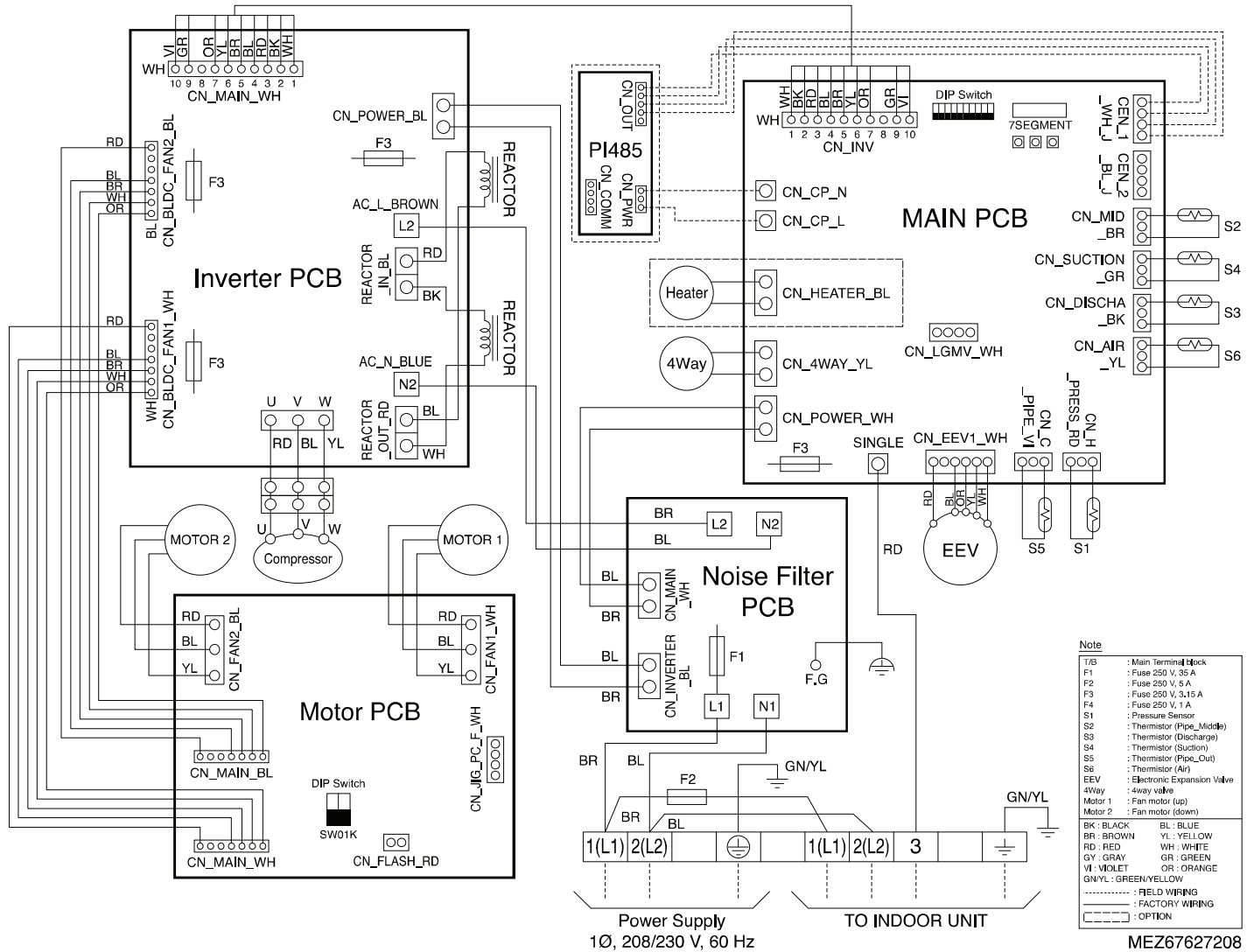
Figure 32: Outdoor Unit Wiring Diagram.
