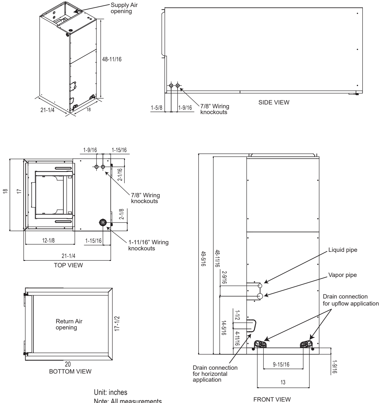
Figure 6: LVN181HV4, LVN241HV4, LVN361HV4 Indoor Unit Dimensions.
