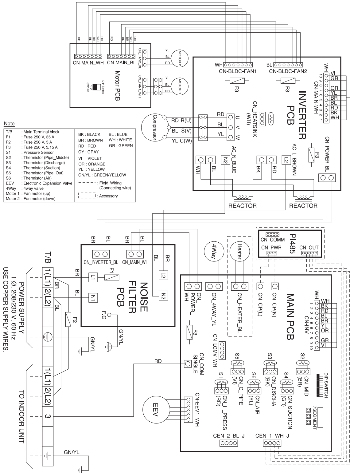
Figure 33: Outdoor Unit Wiring Diagram.
