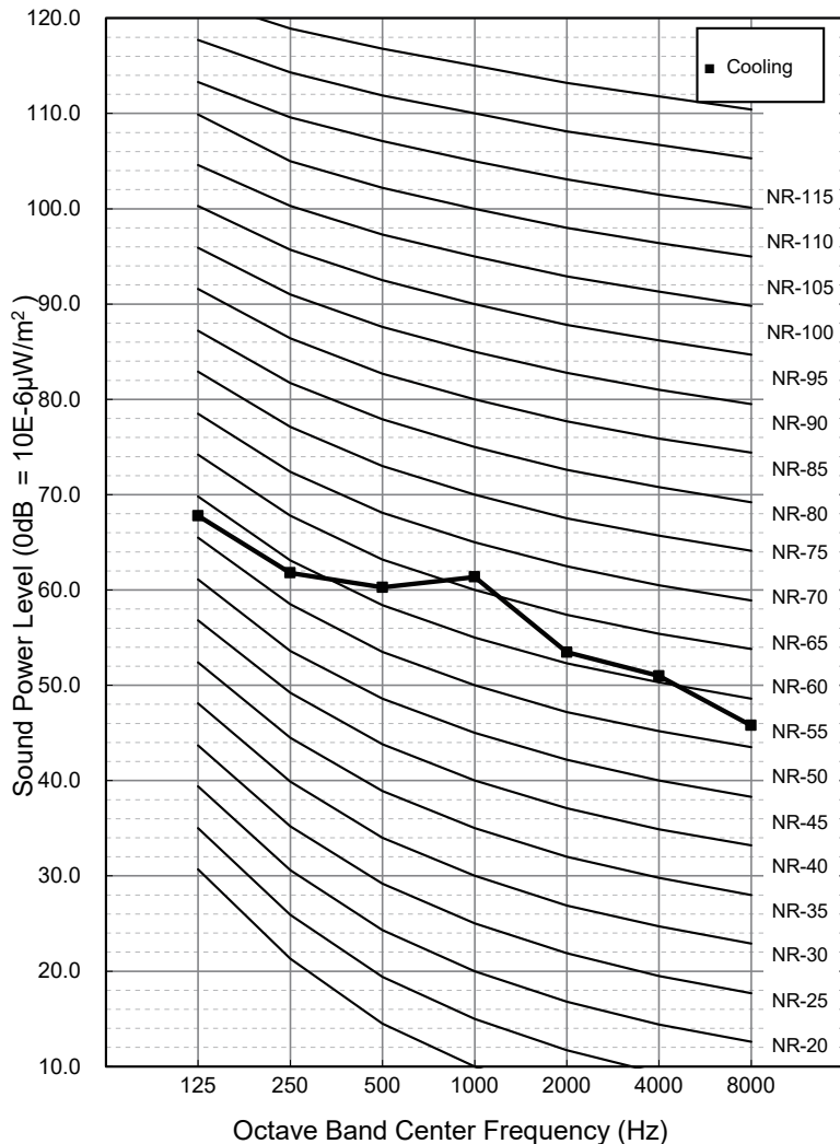
Figure 23: LUU189HV, LUU249HV Sound Power Level Diagram.
