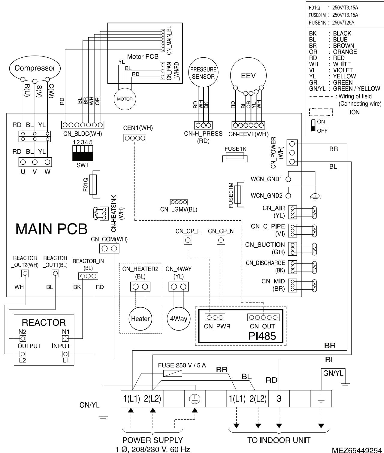
Figure 30: Outdoor Unit Wiring Diagram.
