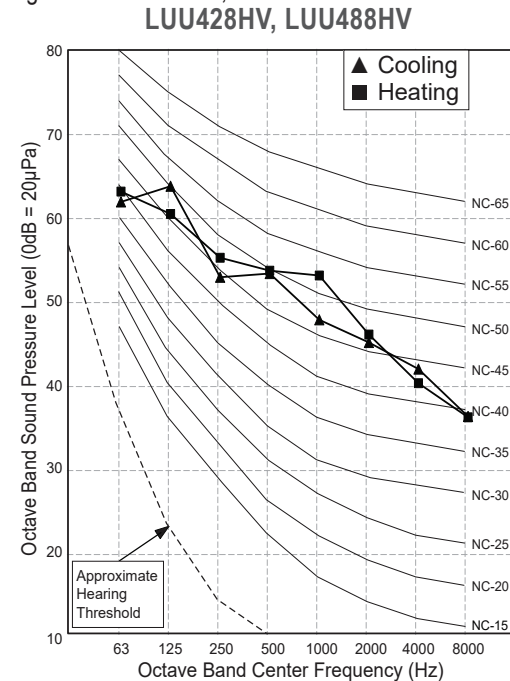
Figure 22: LUU428HV, LUU488HV Sound Pressure Level Diagram.
