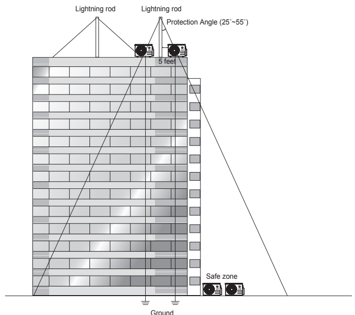
Figure 25: Lightning Protection Diagram.
