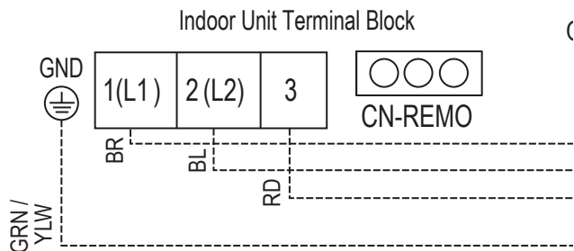
Figure 16: Wired Controller Connection on the Indoor Unit Terminal Block.
