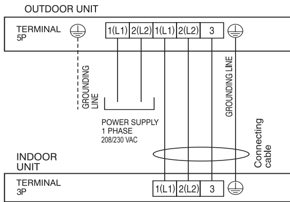
Figure 13: LS090-120HSV5 System Electrical Connections.
