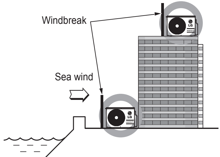
Figure 26: Oceanside Placement Using Windbreak.
