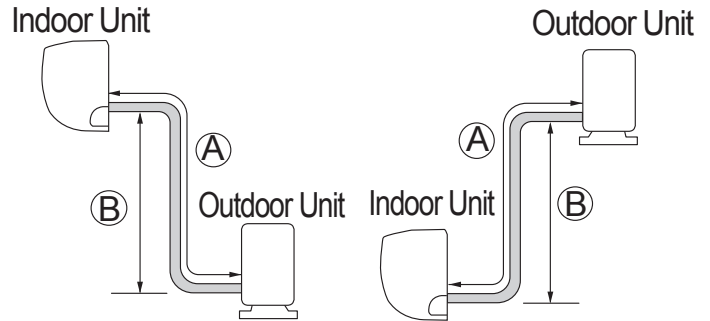
Figure 33: Single Zone High Efficiency Wall Mount System Layout.
