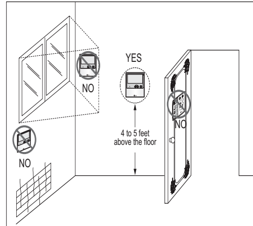
Figure 18: Proper Location for the Wired Controller.
