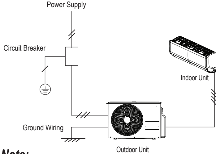
Figure 11: LS090HSV5 and LS120HSV5 General Power / Communications System Schematic.
