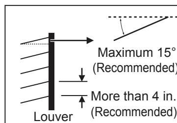
Figure 29: Louver Recommendations.
