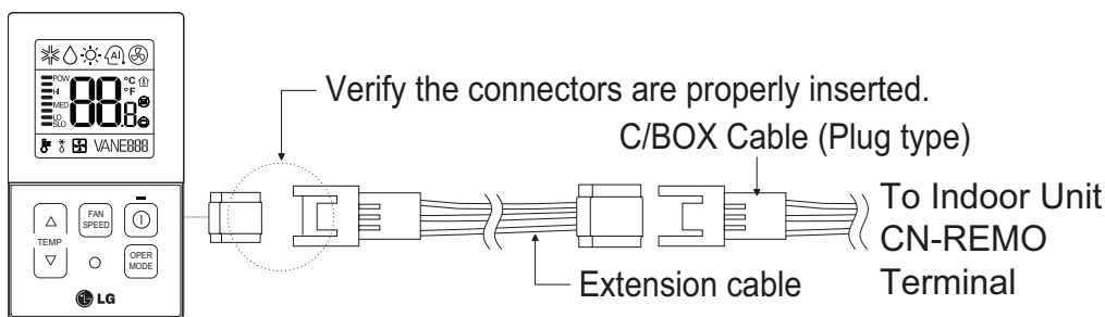
Figure 15: PZCWRC1 LG Wired Remote Extension Cable.
