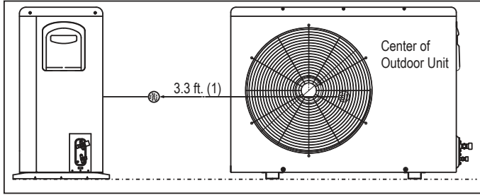
Figure 8: High Efficiency Standard Wall Mount Outdoor Unit Sound Level Measurement.
