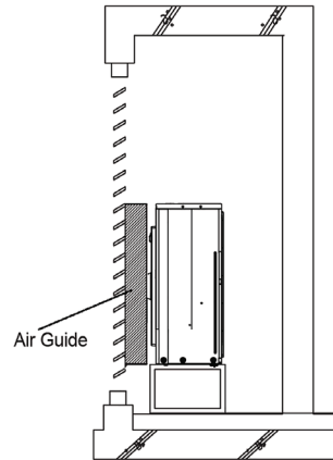
Figure 32: Example of Installing Outdoor Unit Indoors.
