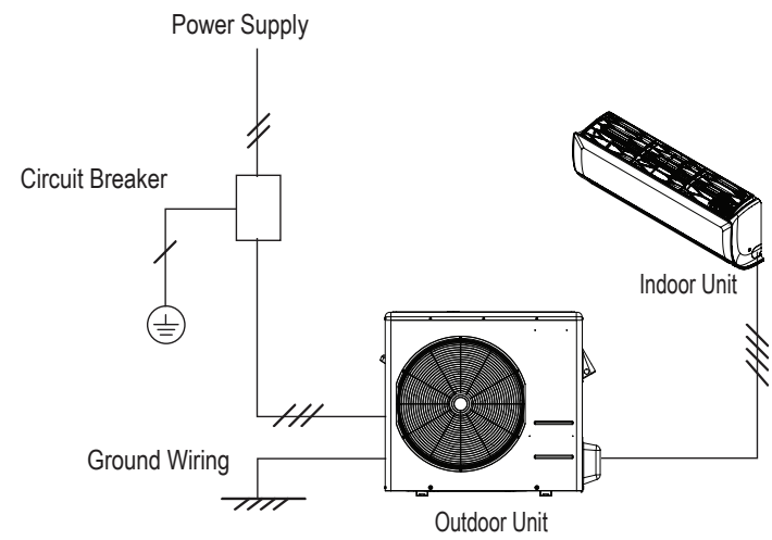
Figure 12: LS180HSV5 General Power / Communications System Schematic.
