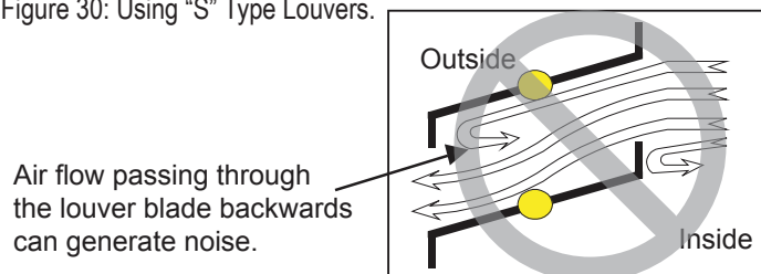
Figure 30: Using “S” Type Louvers.
