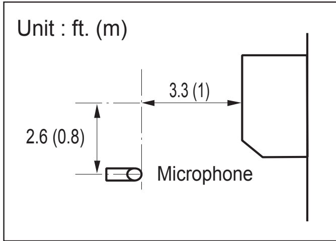
Figure 5: High Efficiency Standard Wall Mount Indoor Unit Sound Level Measurement.
