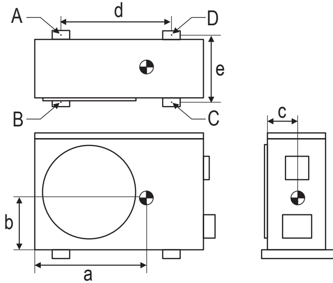
Figure 4: LSU090-120-180HSV5 Outdoor Unit Corner Weight and Center of Gravity Dimensions.
