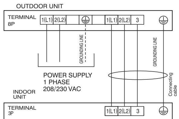
Figure 14: LS180HSV5 System Electrical Connections.
