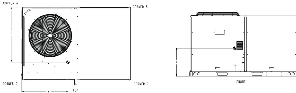
Fig. 9 – Dimensions RGS150
