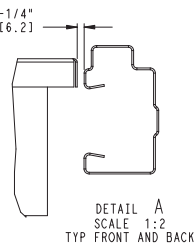
DETAIL A SCALE 1:2 TYP FRONT AND BACK
