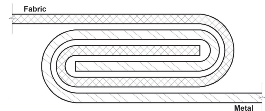
Double Lock Seam – fabric is easily damaged
