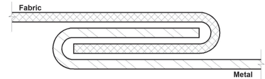
Single Fold Seam – fabric can easily pull out of the connection joint
