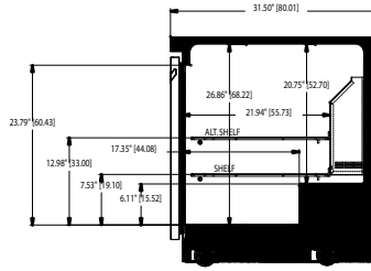
UC4460N Right Side View
