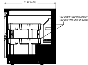
UCD4460N Right Side View
