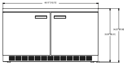
UC4460N Elevation View
