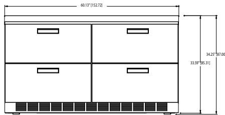
UCD4460N Elevation View
