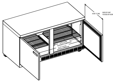
UC4460N ISO View
