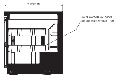
D4448N Right Side View
