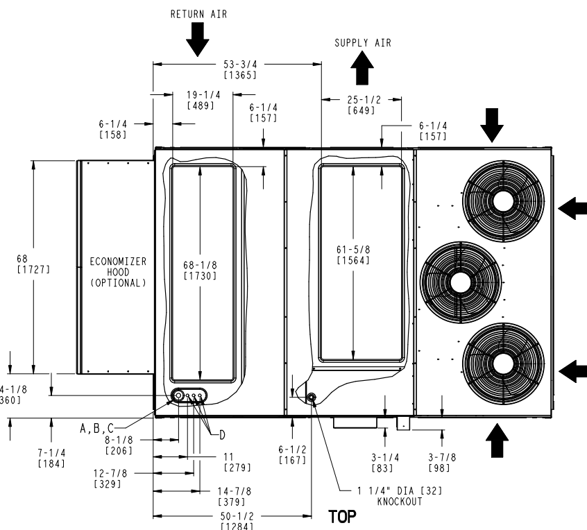
(HORIZONTAL DISCHARGE W/ ECON) (WHEN ORDERED)
