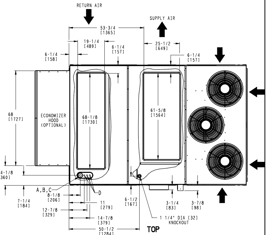
(HORIZONTAL DISCHARGE W/ ECON) (WHEN ORDERED)
