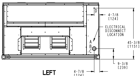
LEFT (HORIZONTAL DISCHARGE W/ ECON) (WHEN ORDERED)
