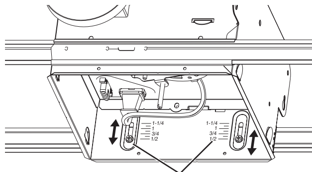
ADJUSTMENT SCREWS
