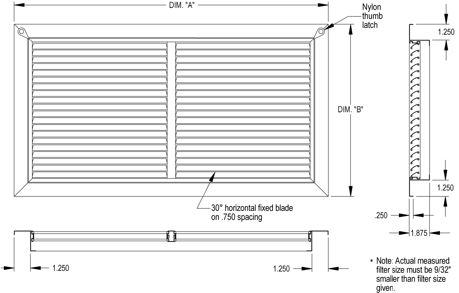
Grille Size and Filter Chart
