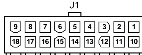
Figure 6. Dome Temperature Sensor Pin 1 & 10 (Red)
