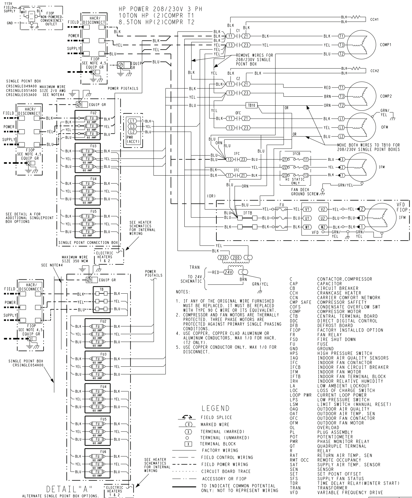
RHS120 TYPICAL POWER WIRING DIAGRAM (208/230-3-60 UNIT SHOWN)
