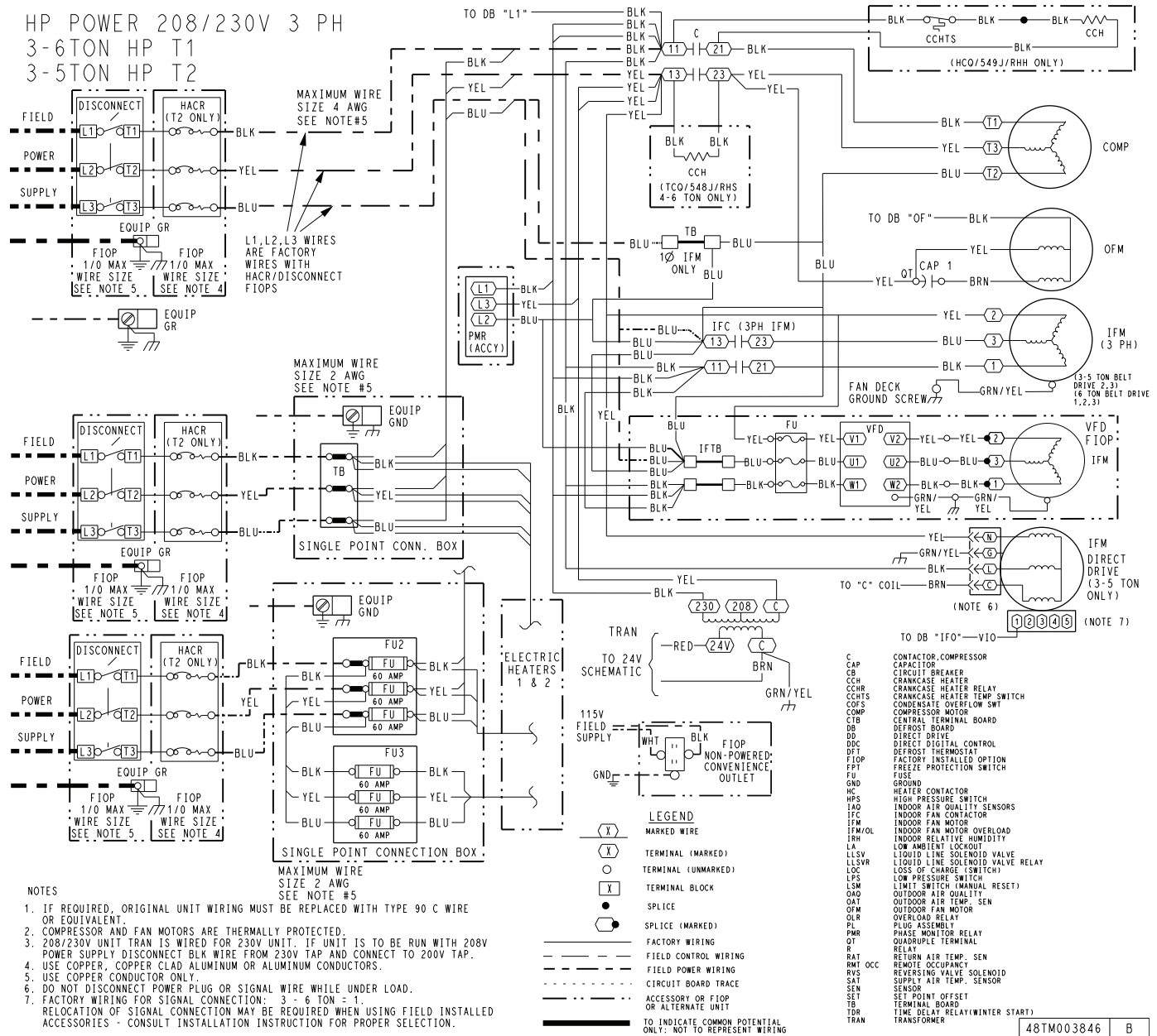
RHS072 TYPICAL POWER WIRING DIAGRAM (208/230-3-60 UNIT SHOWN)
